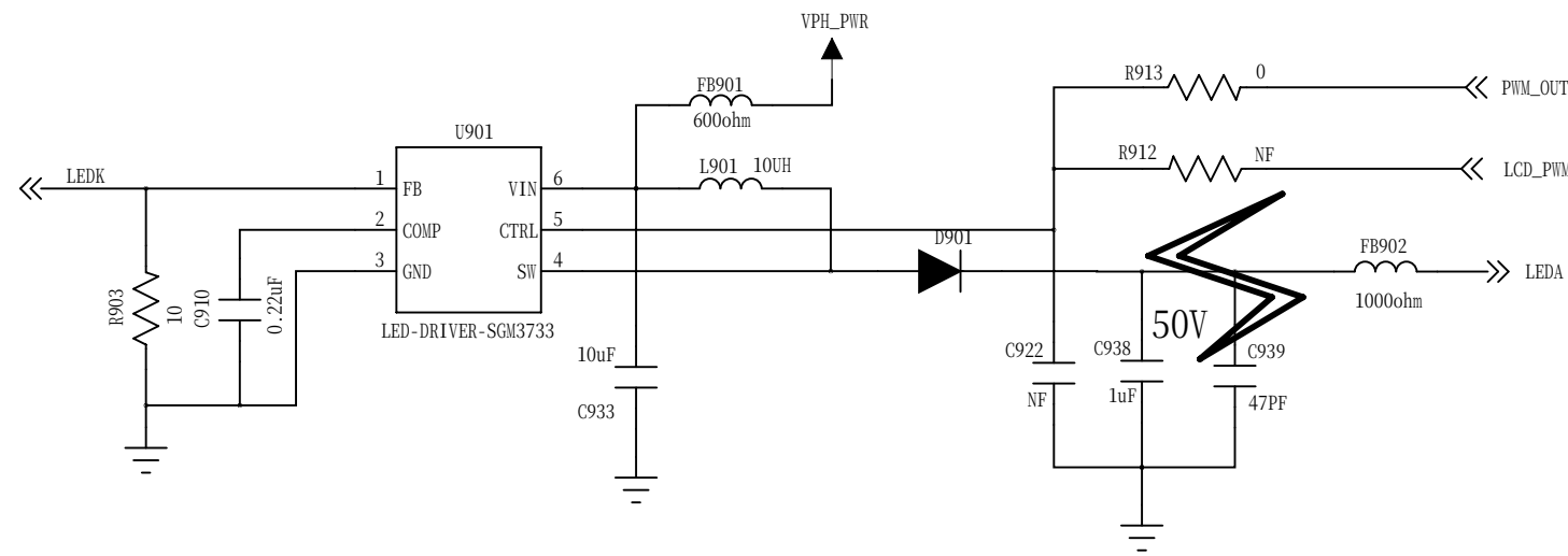
Backlight LED Driver
